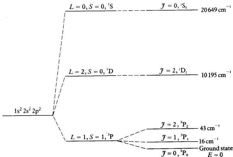
7.8 The splitting of the ground state configuration of carbon.
